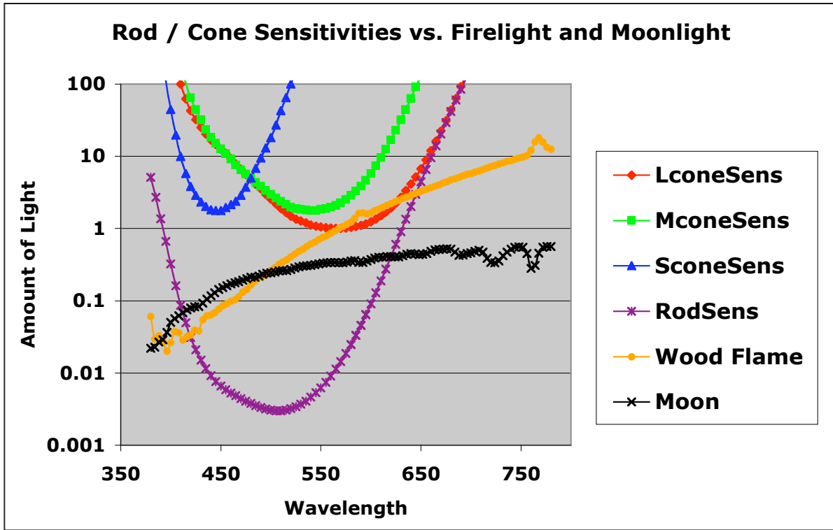
Figure 5 plots the reciprocal Long-, Middle, and Short-wave cone fundamentals from Stockman and Sharpe. In addition, it plots the reciprocal of the scotopic sensitivity for the spectral shape of rod threshold. The LconeSens and The Wood Flame measurements are normalized at 568nm. The Moon measurements were normalized to Wood Flame at 507 nm. Wood Flame has sufficient long-wave light to excite the L-cones. There is sufficient light below 550nm to excite the rods, but not the M- and S-cones. Firelight is an ideal illuminant for rod/cone color vision.
