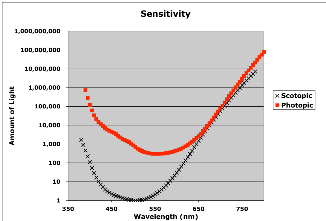
Figure 1 plots the reciprocal of the photopic and scotopic luminosity curves. It plots the amount of light versus wavelength to obtain a threshold response. These curves are usually plotted as sensitivity (1/threshold). Humans are most sensitive to 507nm light at absolute threshold for detection by rods. The photopic standard associated with cone vision is most sensitive at 555nm. The spacing of the two curves is based on experiments that measured the absolute threshold for narrow-band 546nm light and the rod-cone break in the dark-adaptation curve. 2 This data show that the rods are 100 times more sensitive to 546nm light than are the cones.
